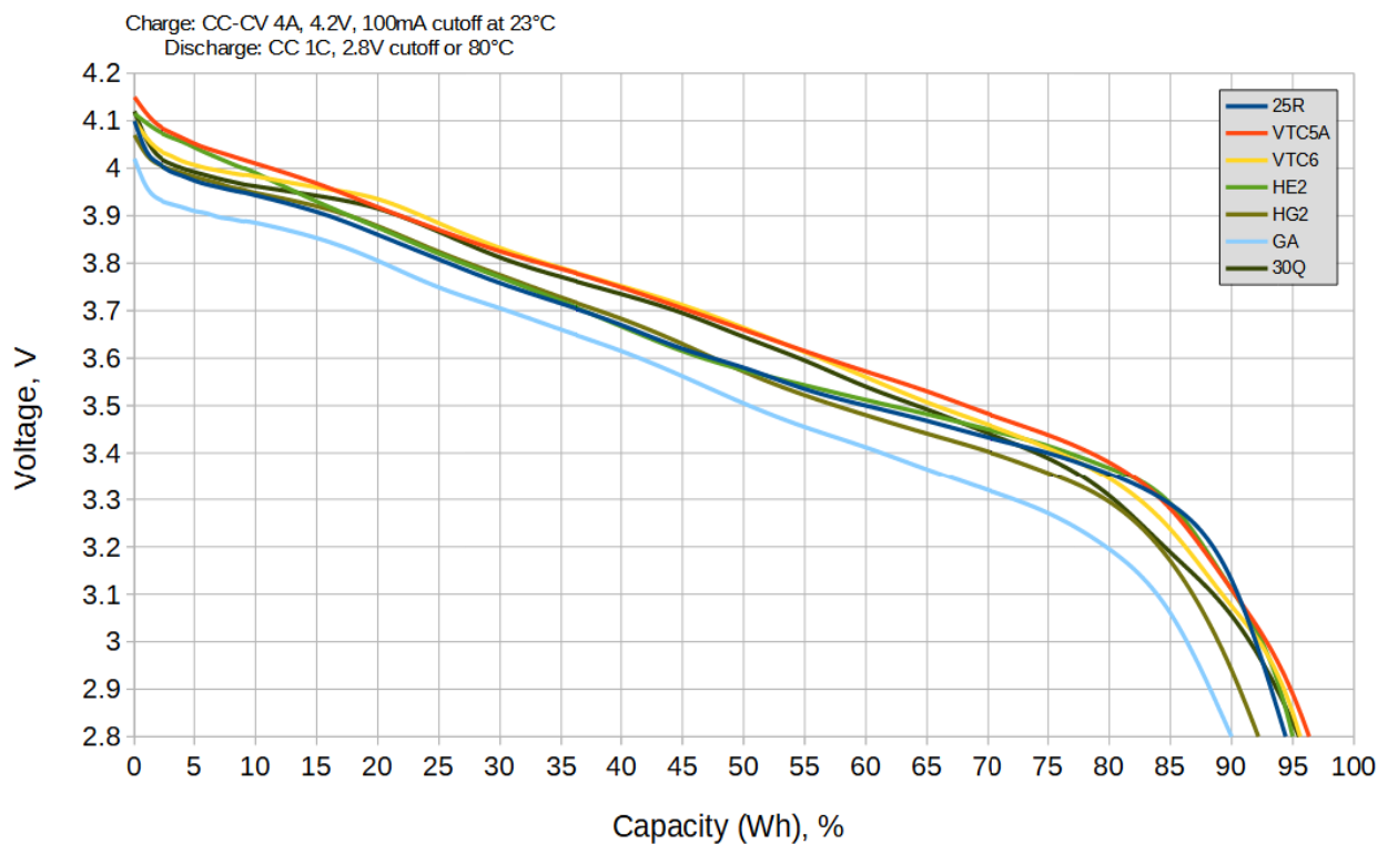
Discharge characteristic at 1C
