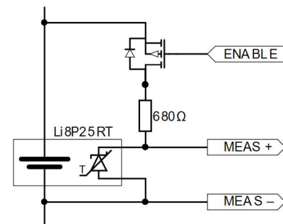
Figure 4: Test circuit.
