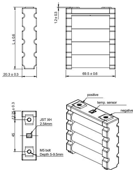
Figure 7: Mechanical dimensions of 1xNp modules
