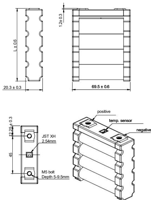
Figure 7: Mechanical dimensions of 1xNp modules
