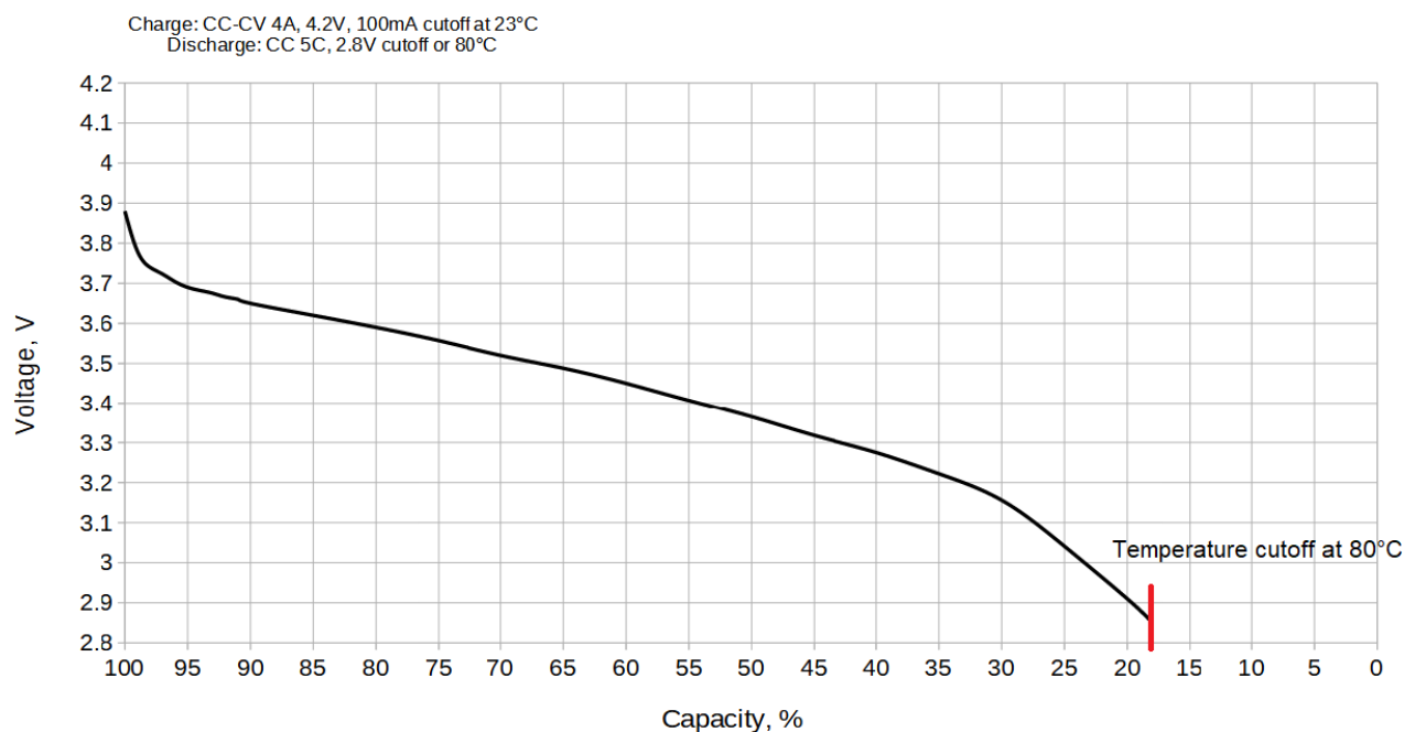
Figure 2: A typical discharge slope at 5C rate.
