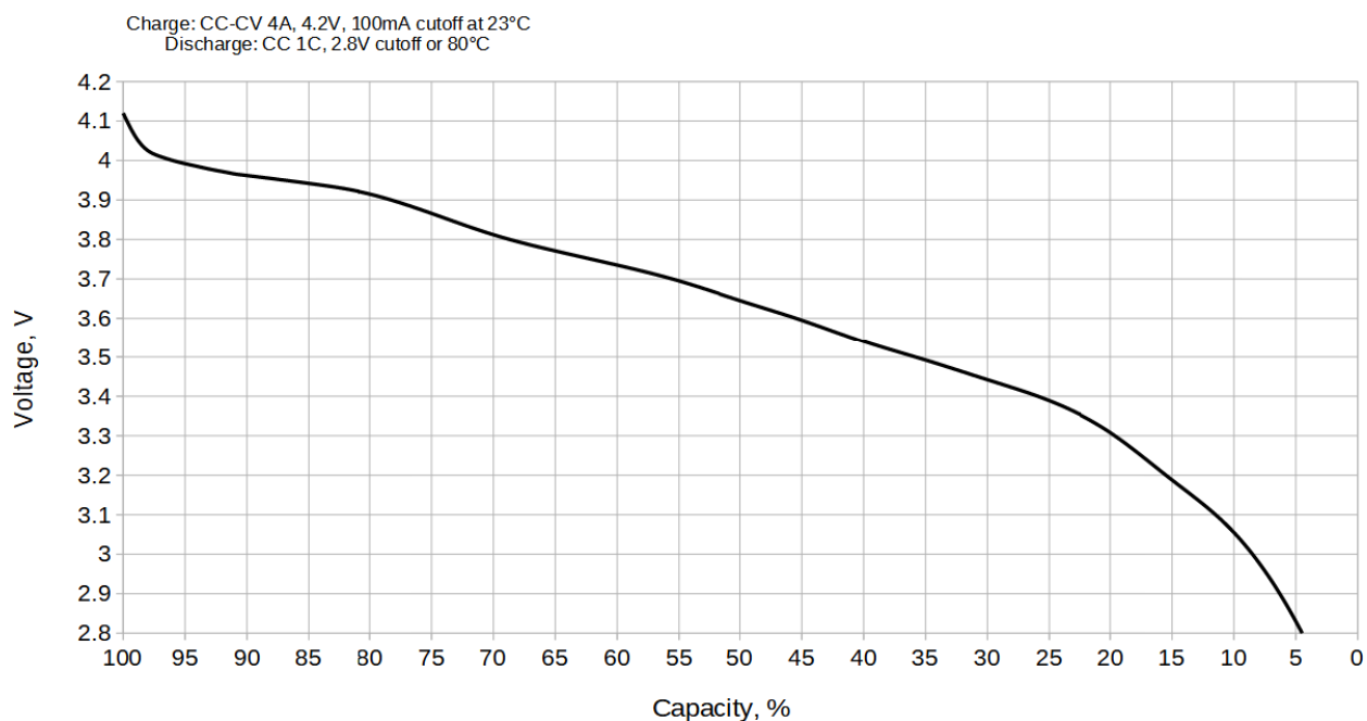
Figure 1: A typical discharge slope at 1C rate.
