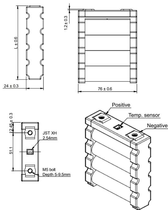
Figure 7: Mechanical dimensions of 1xNp modules
