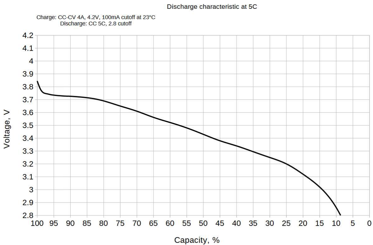
Figure 2: A typical discharge slope at 5C rate.
