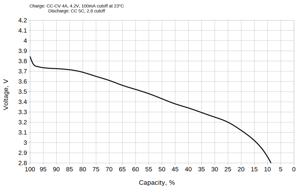
Figure 2: A typical discharge slope at 5C rate.
