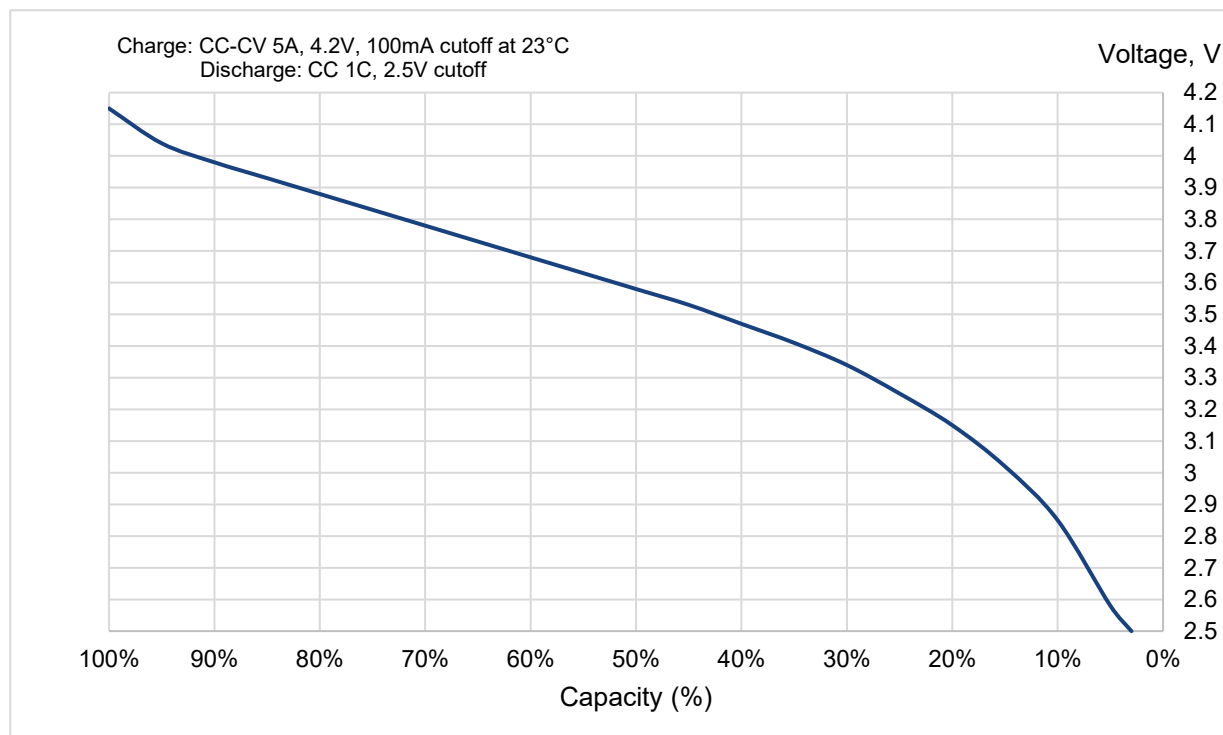
Figure 1: A typical discharge slope at 1C rate.
