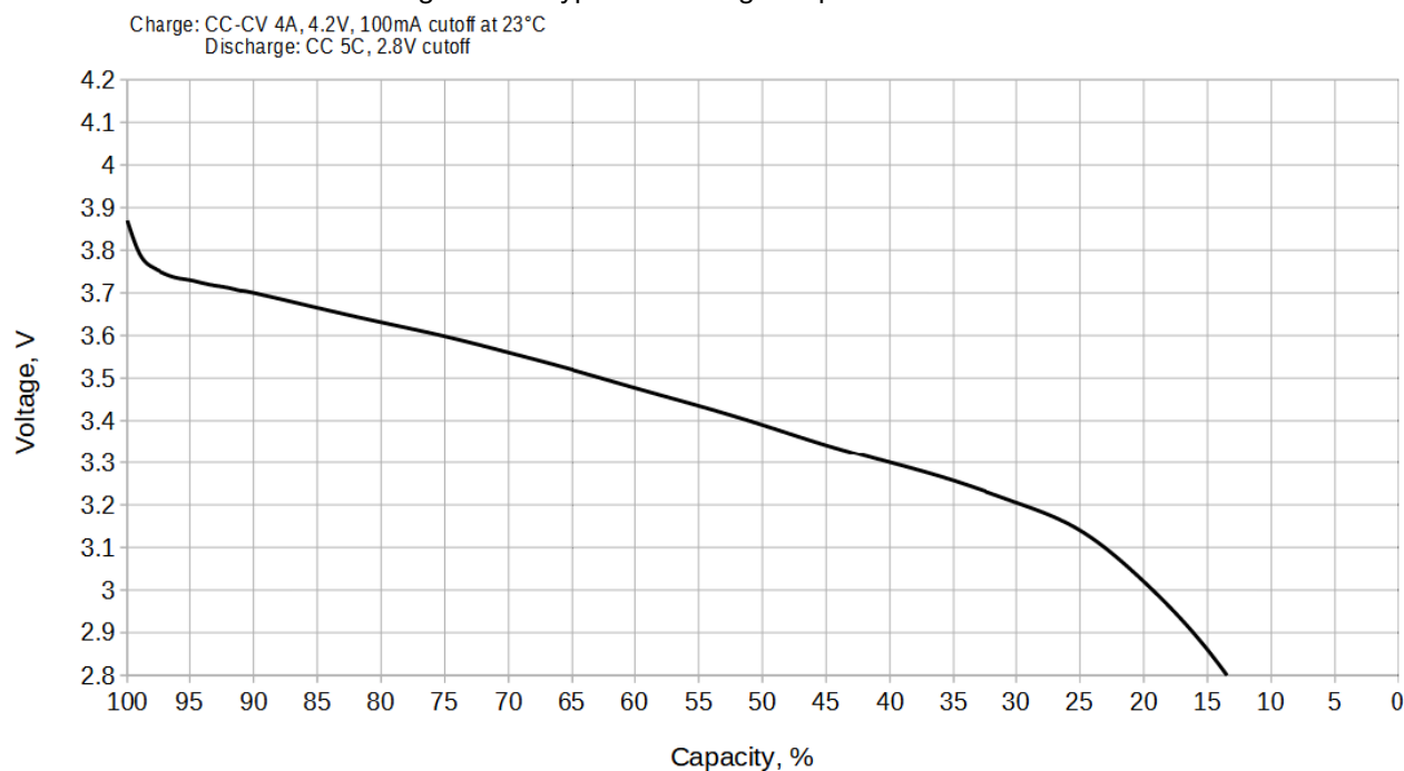
Figure 2: A typical discharge slope at 5C rate.
