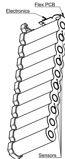
Figure 1: Sensor layout.
