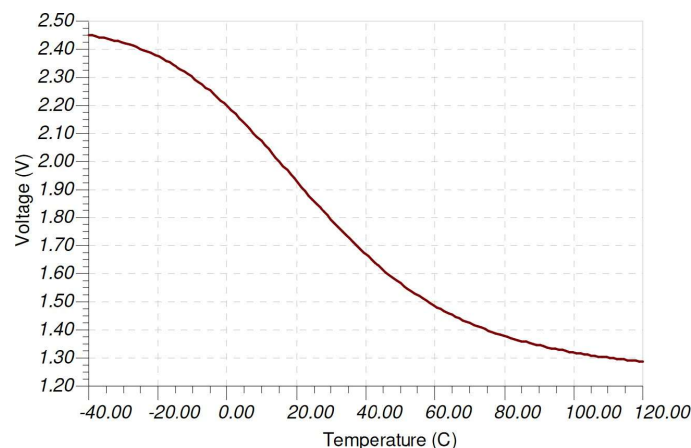
Figure 3: Temperature-Voltage response.
