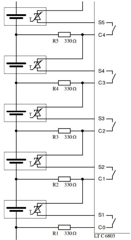
Figure 4: Suggested stack temperature acquisition circuit (simplified).
