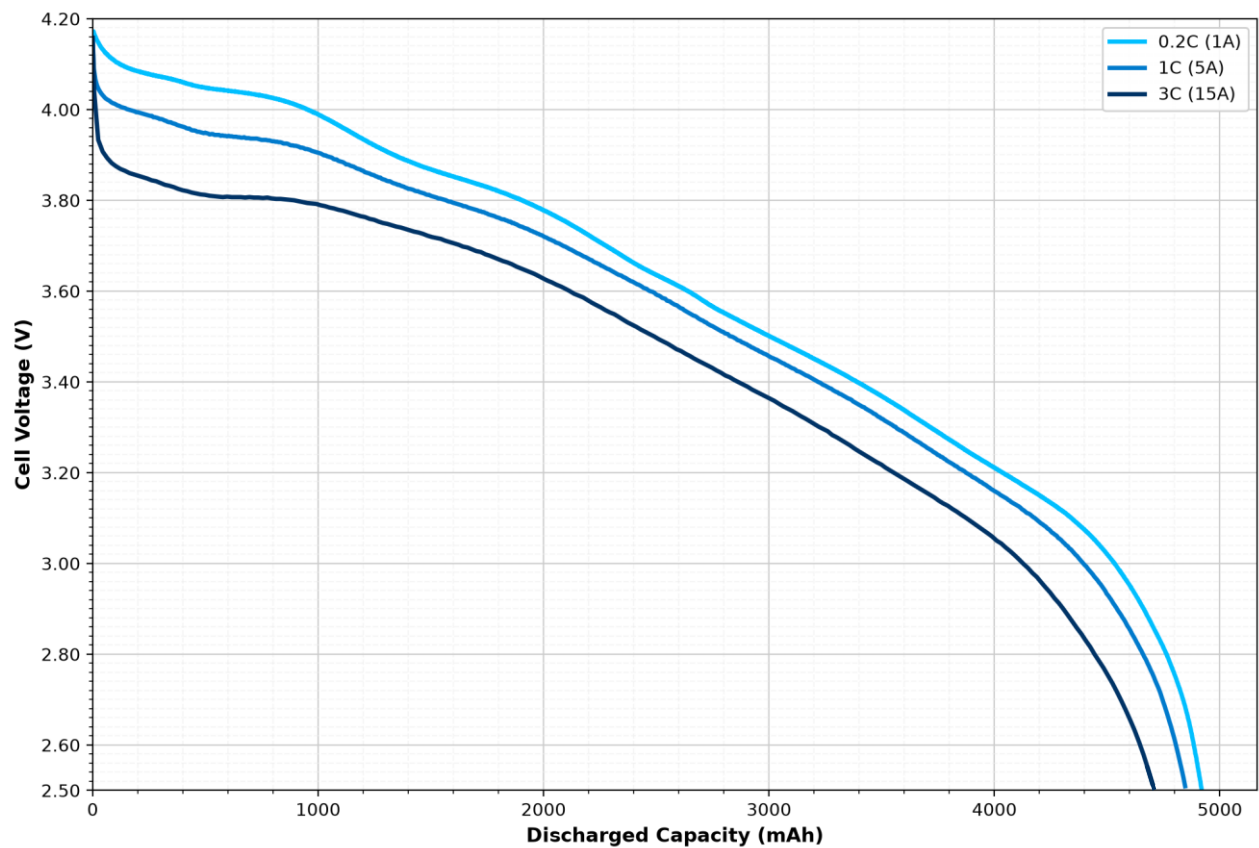
Figure 1: Discharge characteristics of Li1x1pSA124 at different loads
